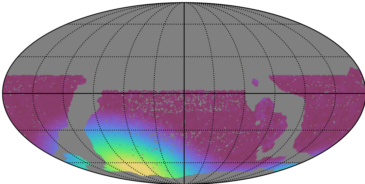
scp_reweight_v3.3_10yrs WFD y band: Min moonDistance
