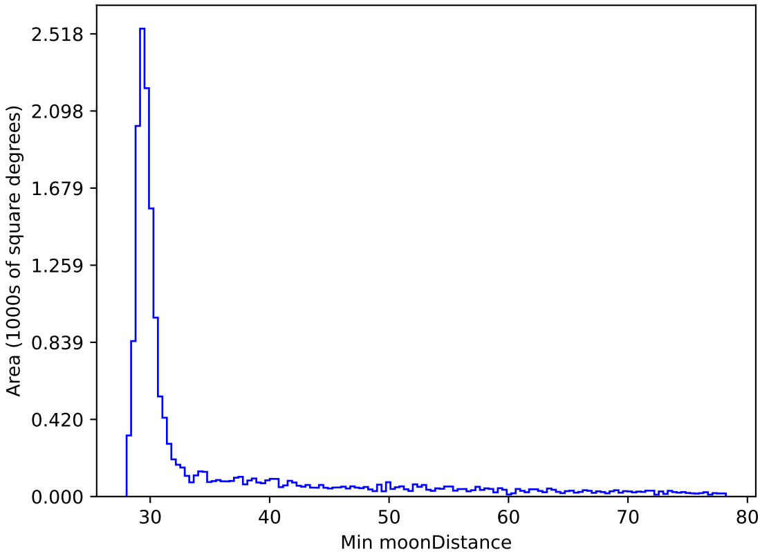
scp_reweight_v3.3_10yrs WFD y band: Min moonDistance
