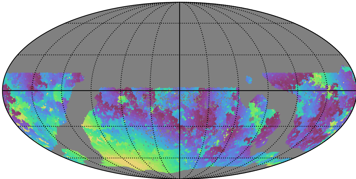
scp_reweight_v3.3_10yrs WFD u band: Min moonDistance
