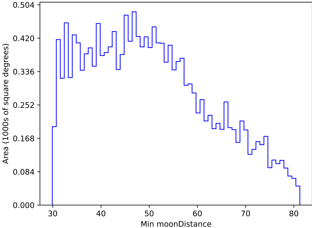
scp_reweight_v3.3_10yrs WFD u band: Min moonDistance
