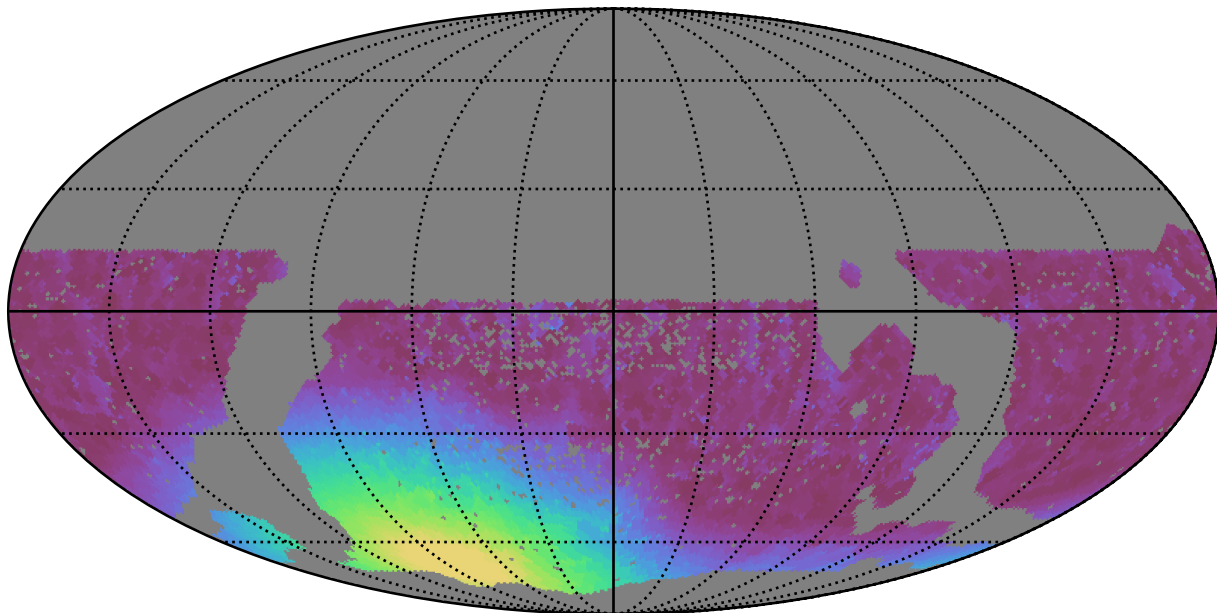
scp_reweight_v3.3_10yrs WFD r band: Min moonDistance
