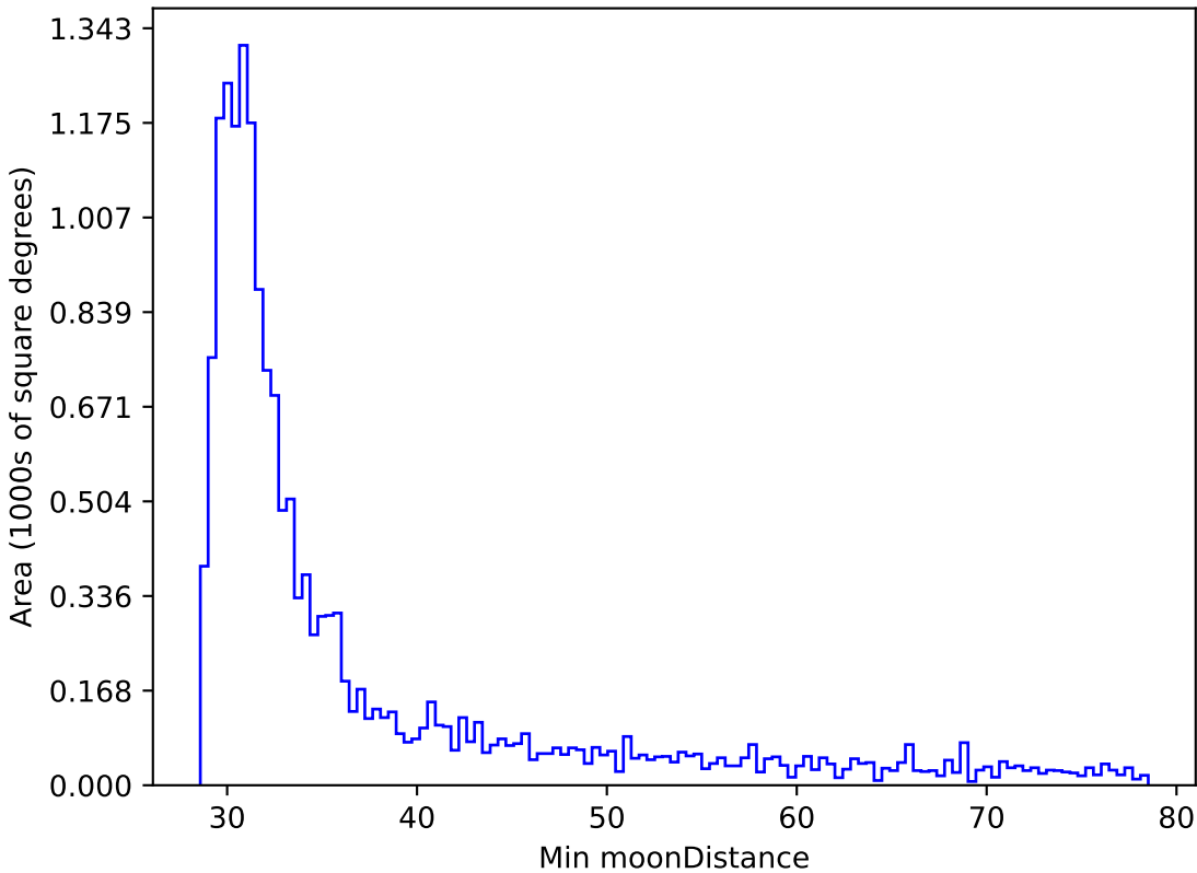
scp_reweight_v3.3_10yrs WFD r band: Min moonDistance
