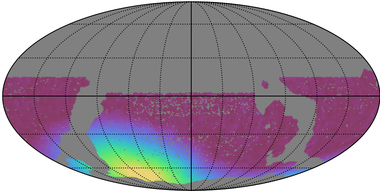
scp_reweight_v3.3_10yrs WFD i band: Min moonDistance
