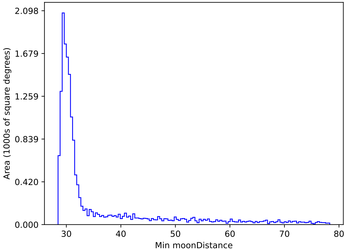
scp_reweight_v3.3_10yrs WFD i band: Min moonDistance
