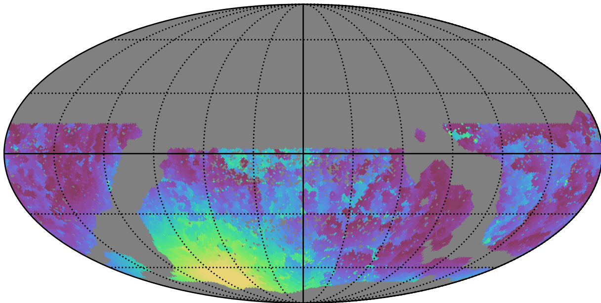
scp_reweight_v3.3_10yrs WFD g band: Min moonDistance
