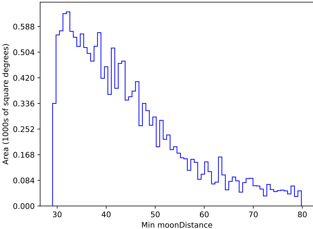
scp_reweight_v3.3_10yrs WFD g band: Min moonDistance
