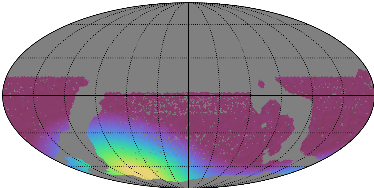
scp_reweight_v3.3_10yrs WFD all bands: Min moonDistance
