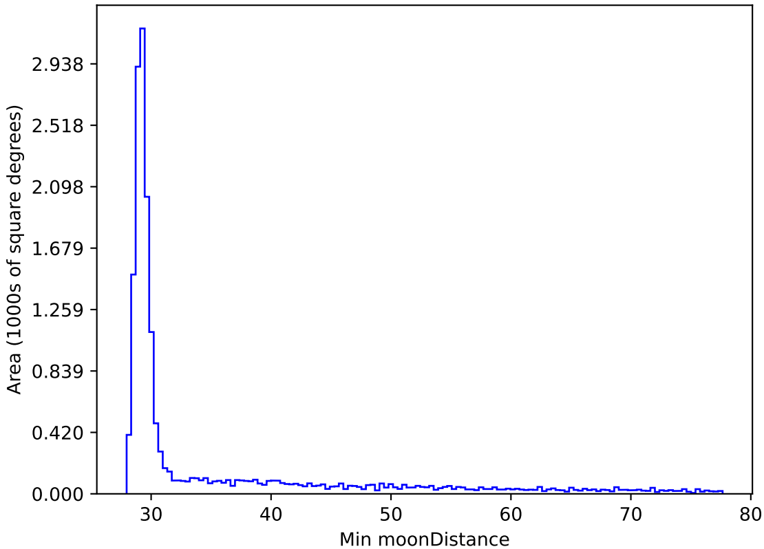
scp_reweight_v3.3_10yrs WFD all bands: Min moonDistance
