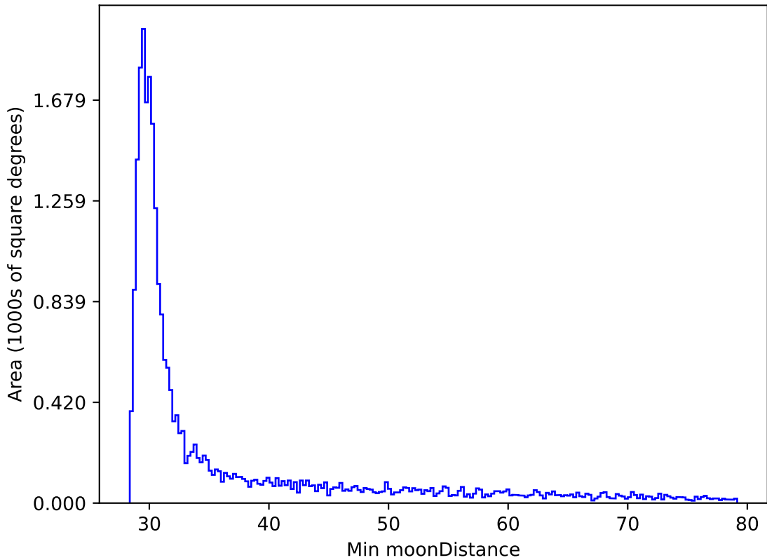
scp_reweight_v3.3_10yrs All sky z band: Min moonDistance
