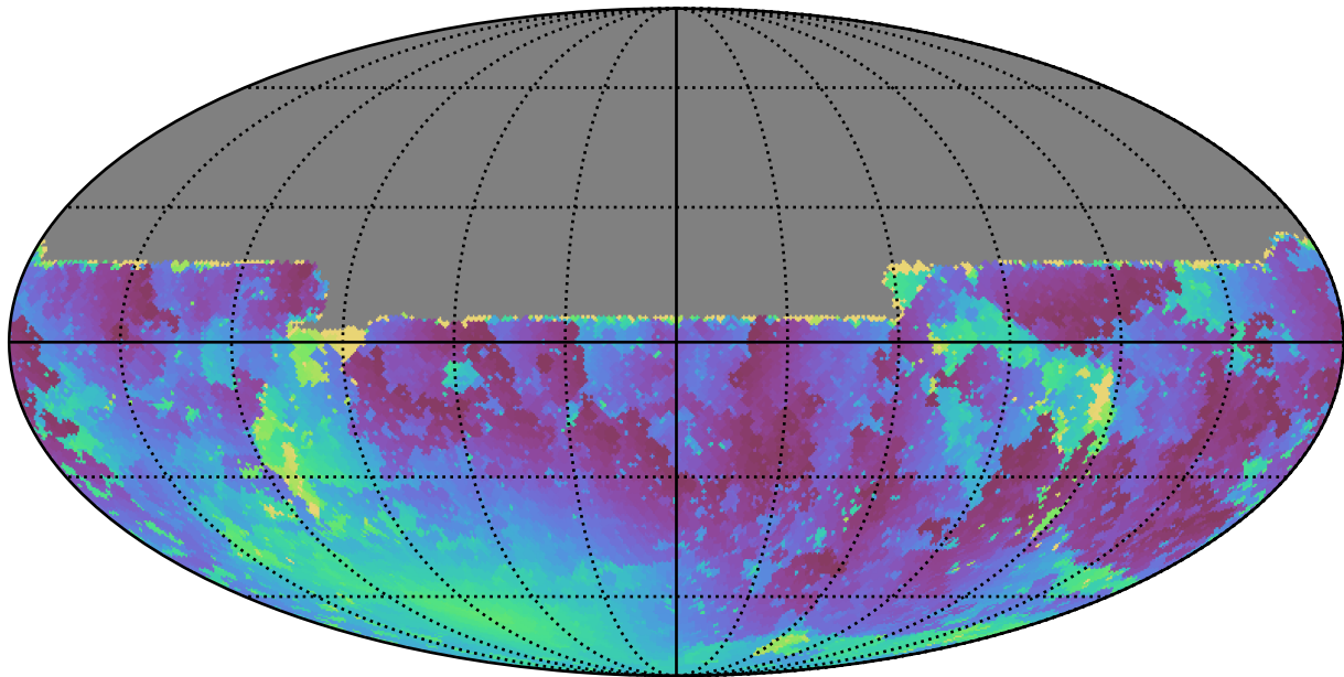
scp_reweight_v3.3_10yrs All sky u band: Min moonDistance
