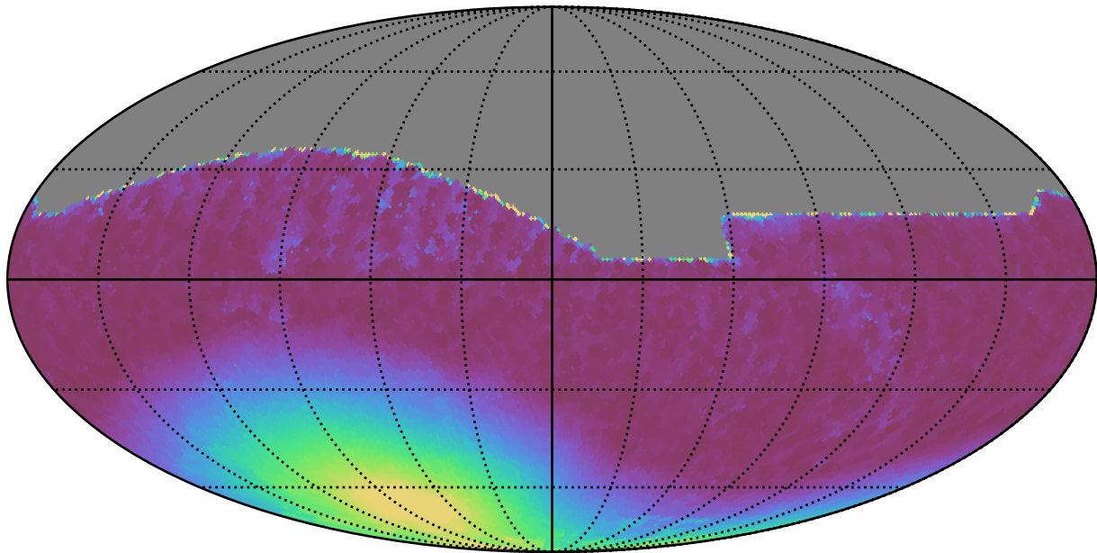
scp_reweight_v3.3_10yrs All sky i band: Min moonDistance
