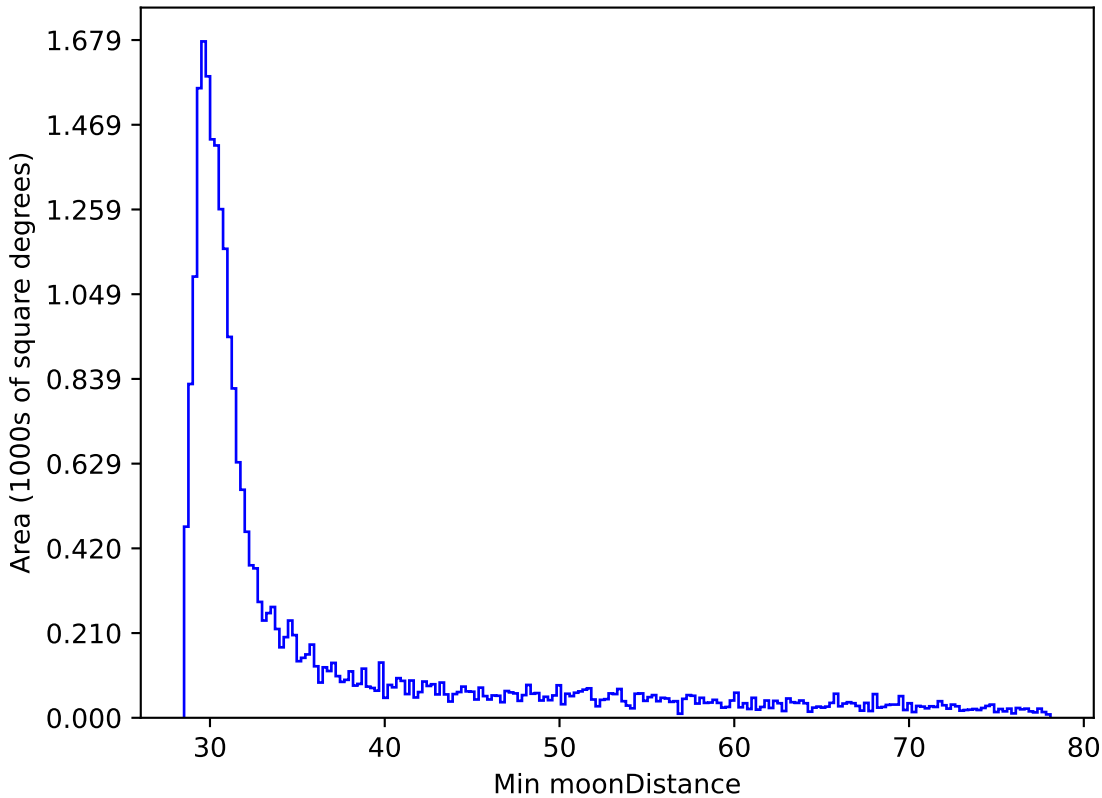
scp_reweight_v3.3_10yrs All sky i band: Min moonDistance
