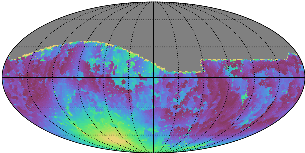
scp_reweight_v3.3_10yrs All sky g band: Min moonDistance
