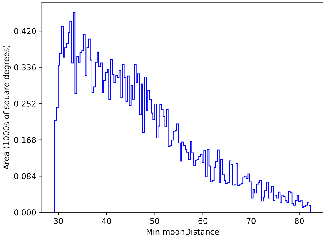
scp_reweight_v3.3_10yrs All sky g band: Min moonDistance
