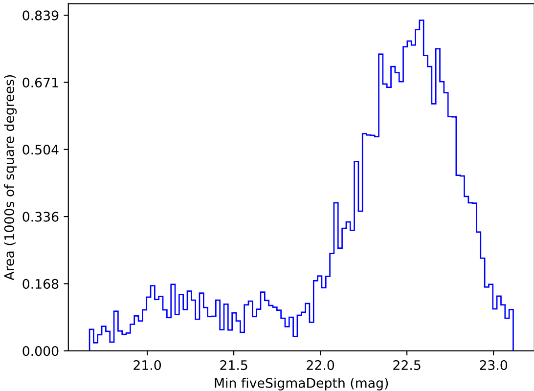
scp_reweight_v3.3_10yrs Yr 1 z band: Min fiveSigmaDepth
