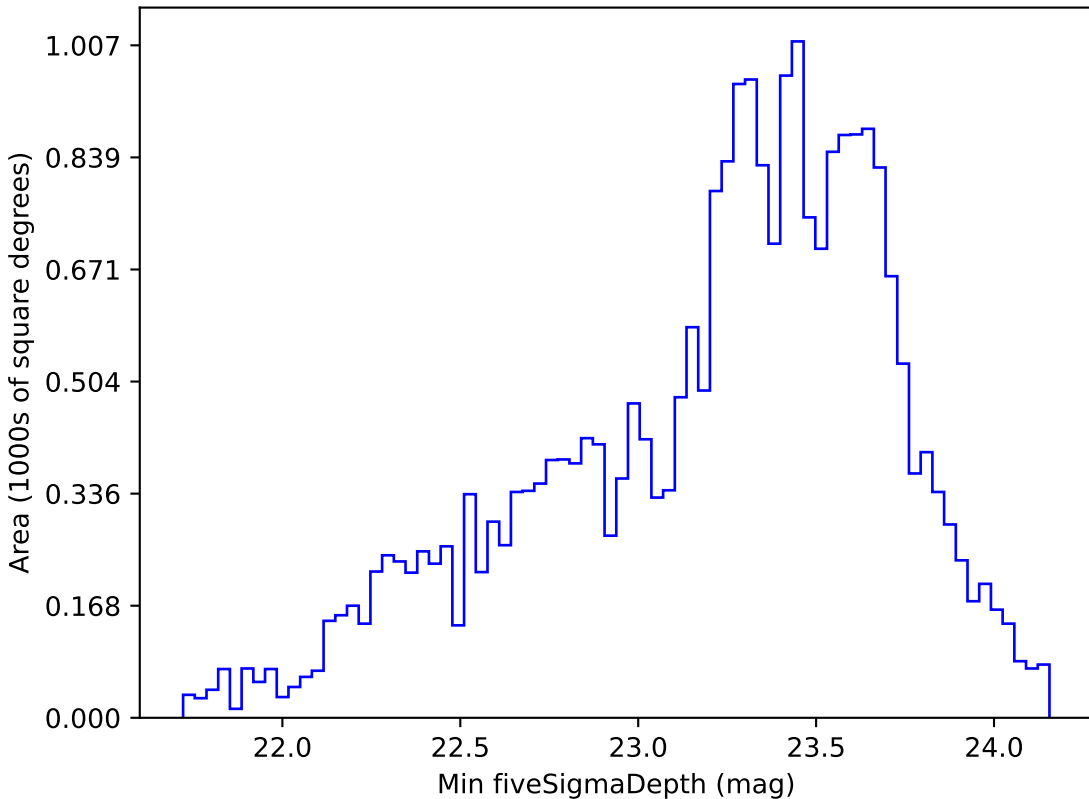
scp_reweight_v3.3_10yrs Yr 1 r band: Min fiveSigmaDepth
