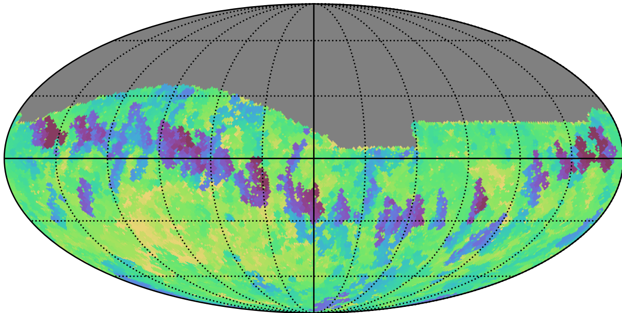
scp_reweight_v3.3_10yrs Yr 1 i band: Min fiveSigmaDepth
