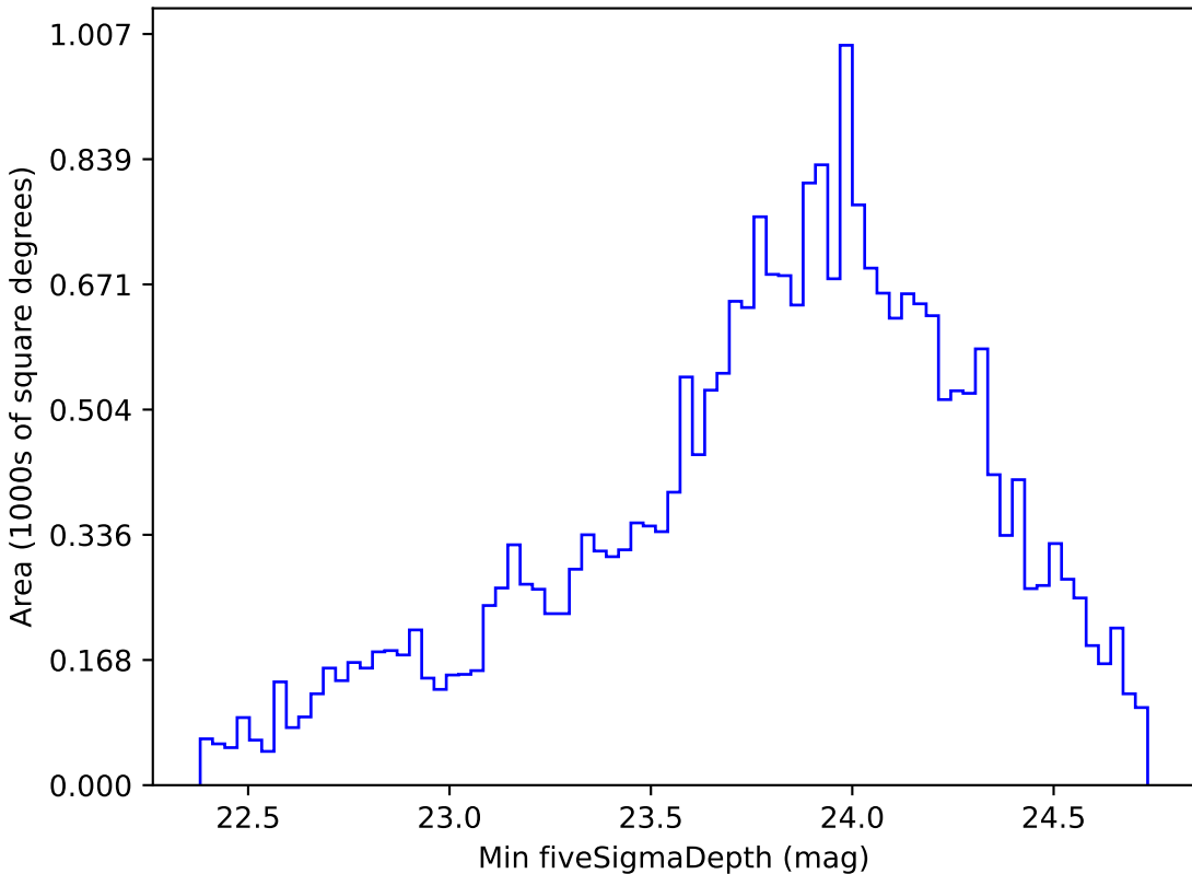
scp_reweight_v3.3_10yrs Yr 1 g band: Min fiveSigmaDepth
