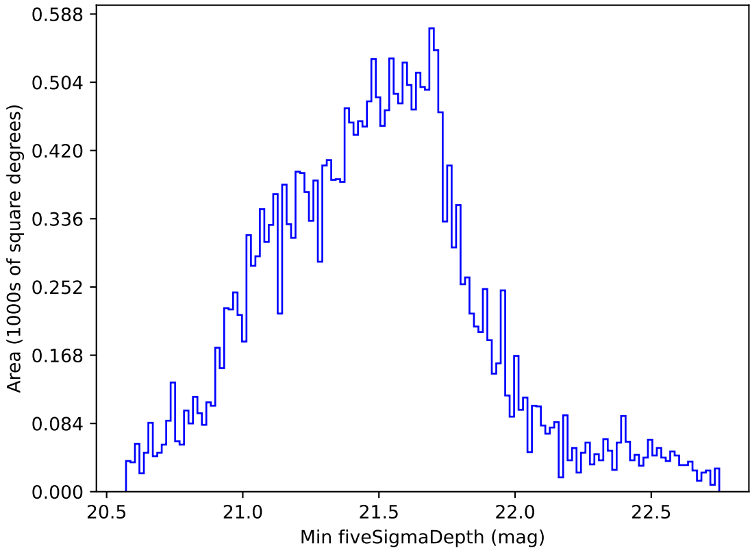
scp_reweight_v3.3_10yrs Yr 1 all bands: Min fiveSigmaDepth
