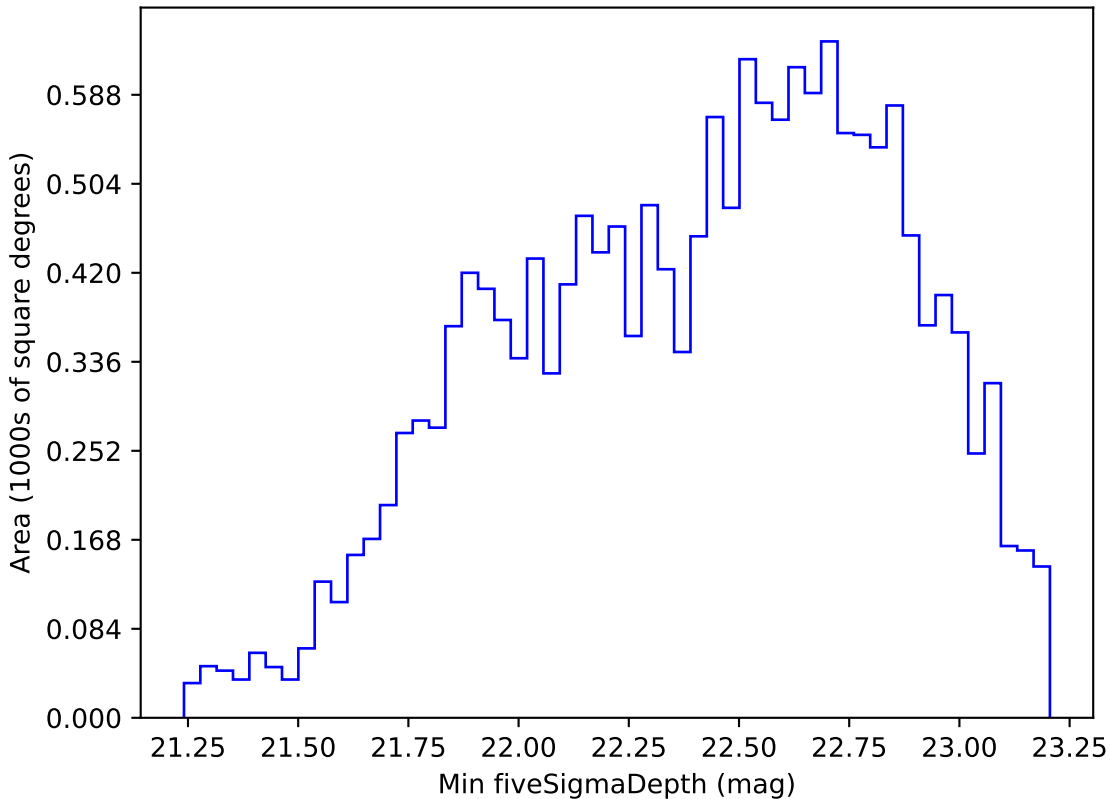
scp_reweight_v3.3_10yrs WFD r band: Min fiveSigmaDepth
