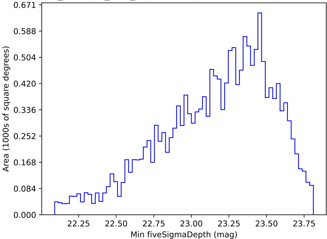
scp_reweight_v3.3_10yrs WFD g band: Min fiveSigmaDepth
