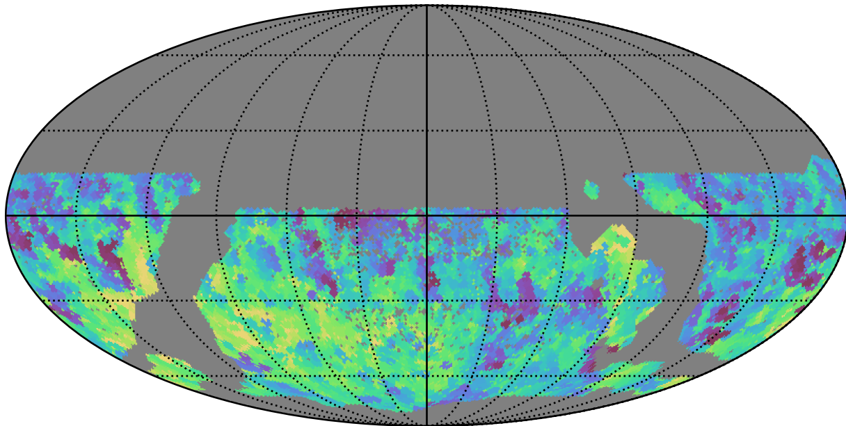
scp_reweight_v3.3_10yrs WFD all bands: Min fiveSigmaDepth
