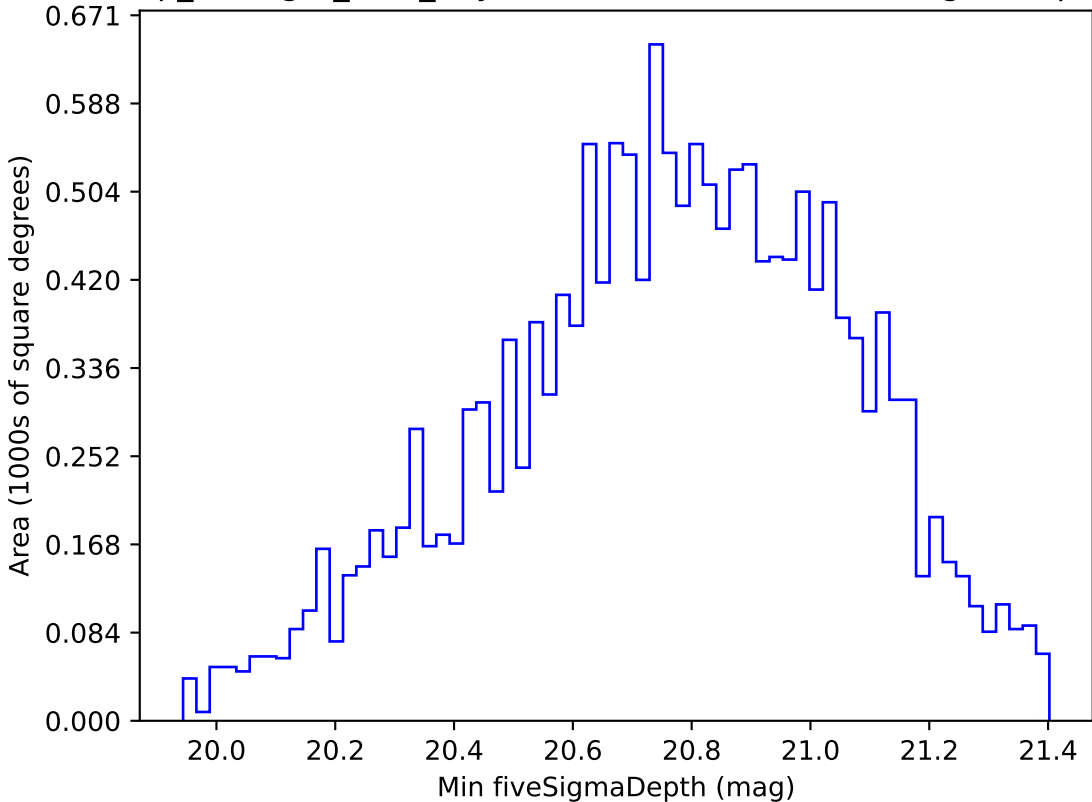
scp_reweight_v3.3_10yrs WFD all bands: Min fiveSigmaDepth
