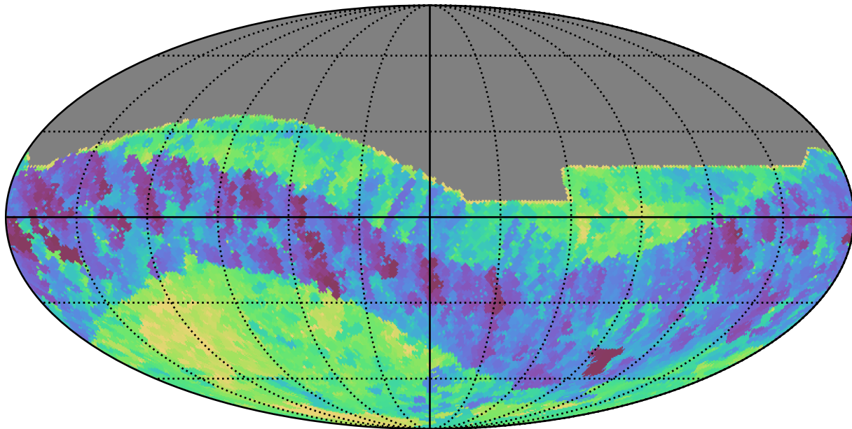
scp_reweight_v3.3_10yrs All sky z band: Min fiveSigmaDepth
