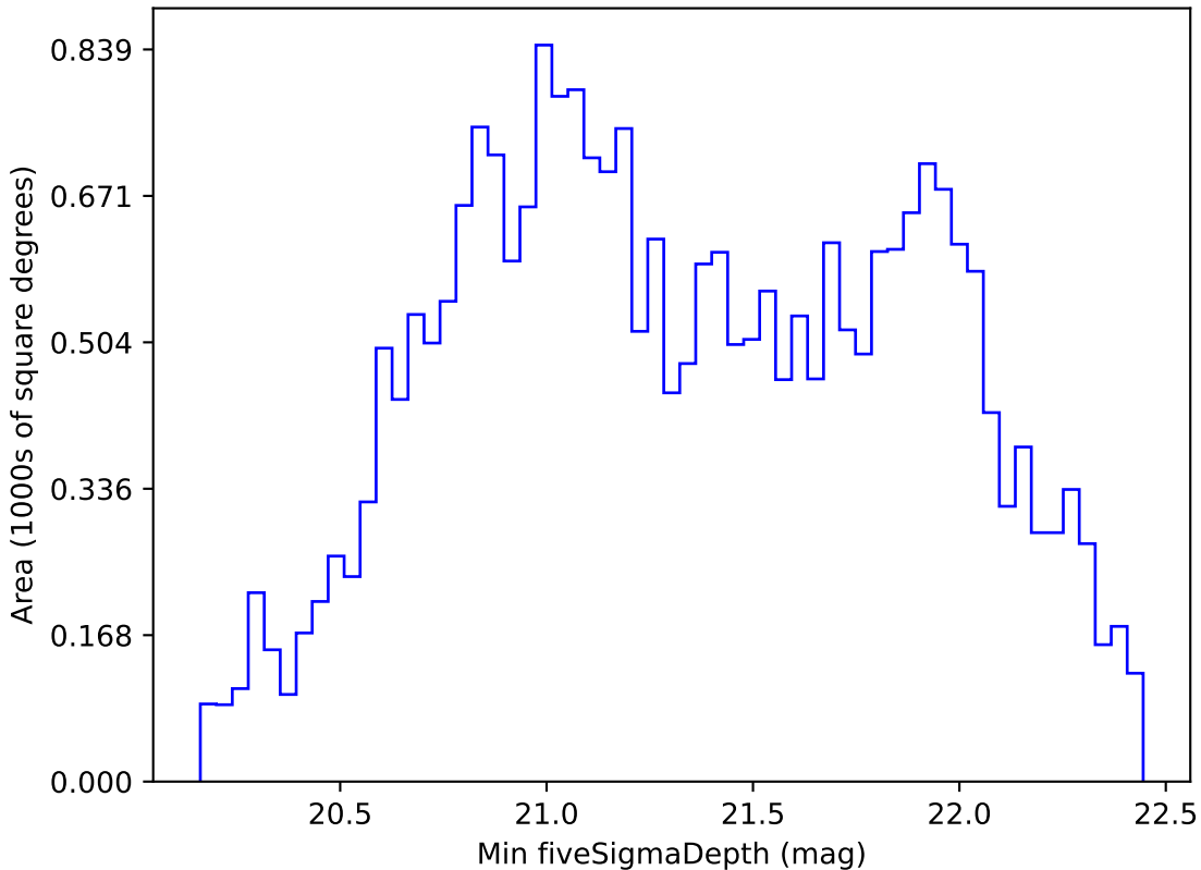
scp_reweight_v3.3_10yrs All sky z band: Min fiveSigmaDepth
