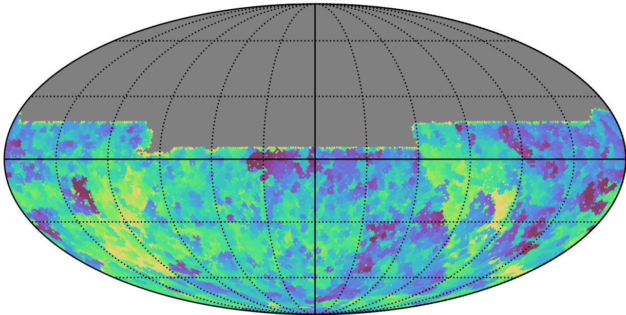
scp_reweight_v3.3_10yrs All sky y band: Min fiveSigmaDepth
