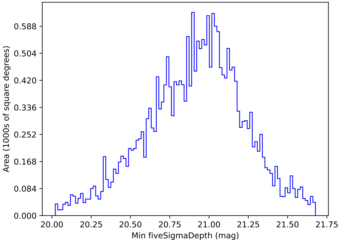
scp_reweight_v3.3_10yrs All sky y band: Min fiveSigmaDepth
