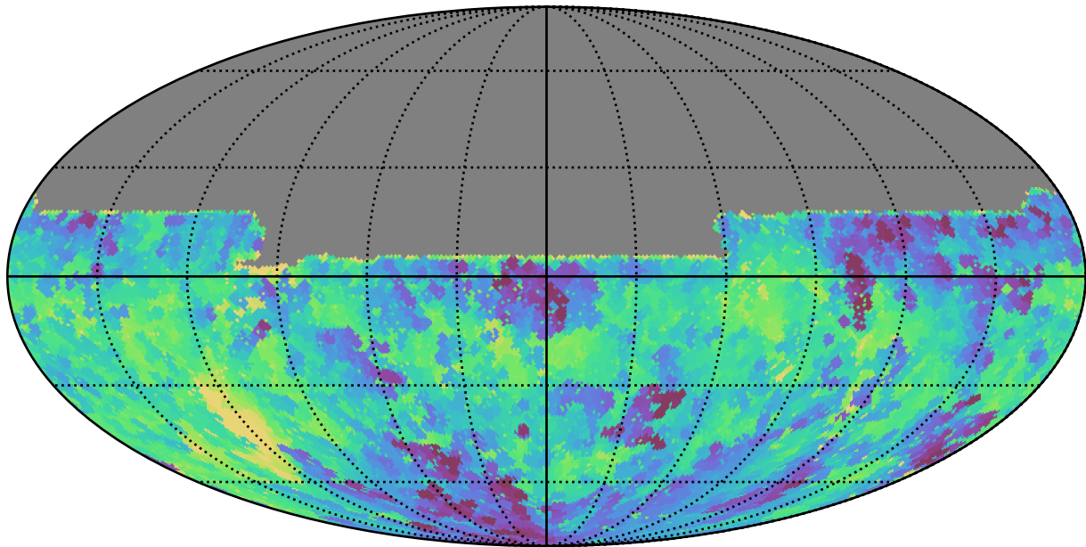
scp_reweight_v3.3_10yrs All sky u band: Min fiveSigmaDepth
