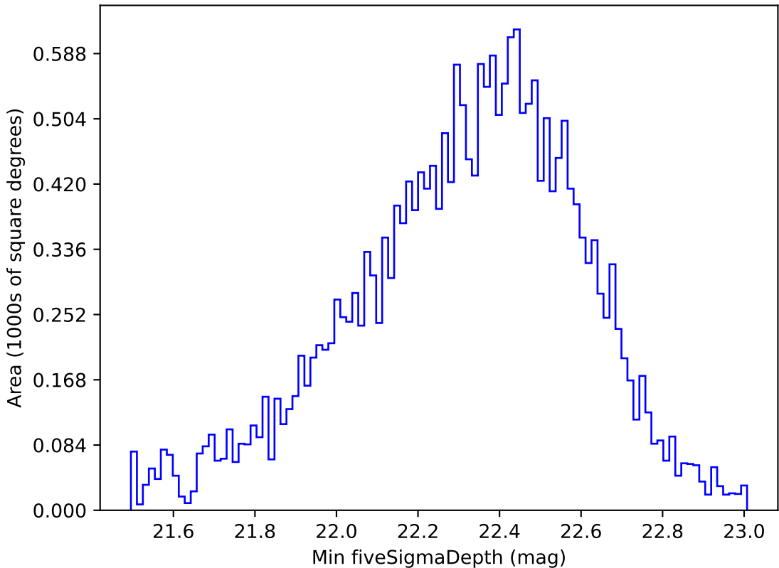
scp_reweight_v3.3_10yrs All sky u band: Min fiveSigmaDepth
