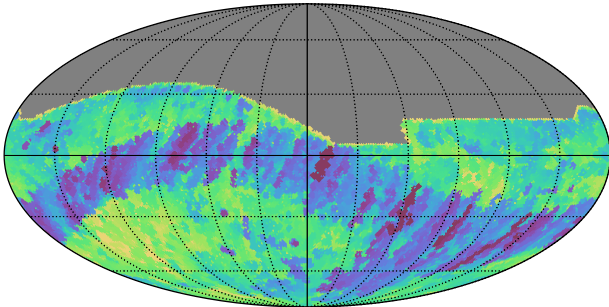
scp_reweight_v3.3_10yrs All sky r band: Min fiveSigmaDepth
