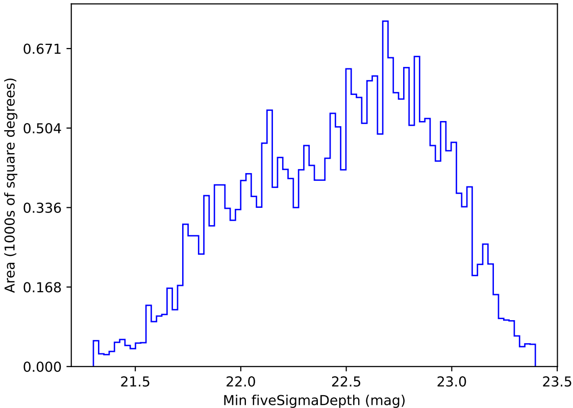
scp_reweight_v3.3_10yrs All sky r band: Min fiveSigmaDepth
