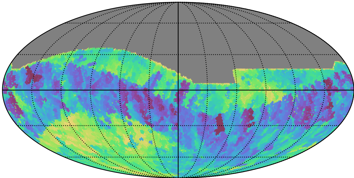
scp_reweight_v3.3_10yrs All sky i band: Min fiveSigmaDepth
