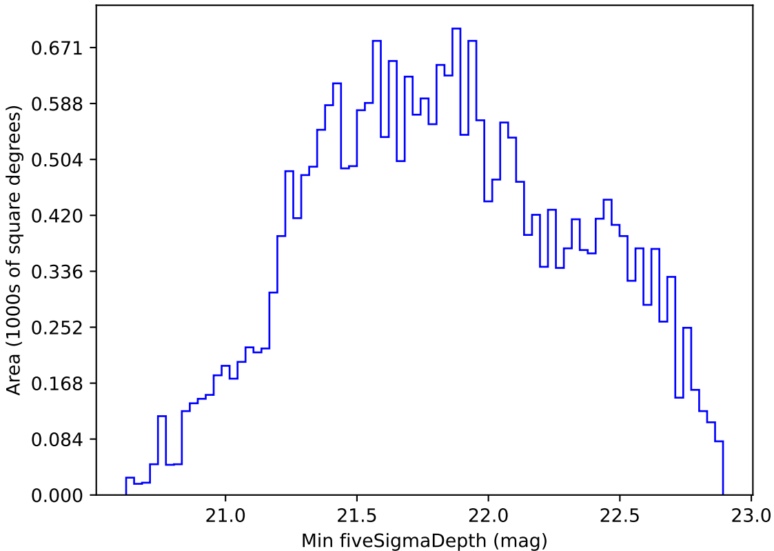
scp_reweight_v3.3_10yrs All sky i band: Min fiveSigmaDepth
