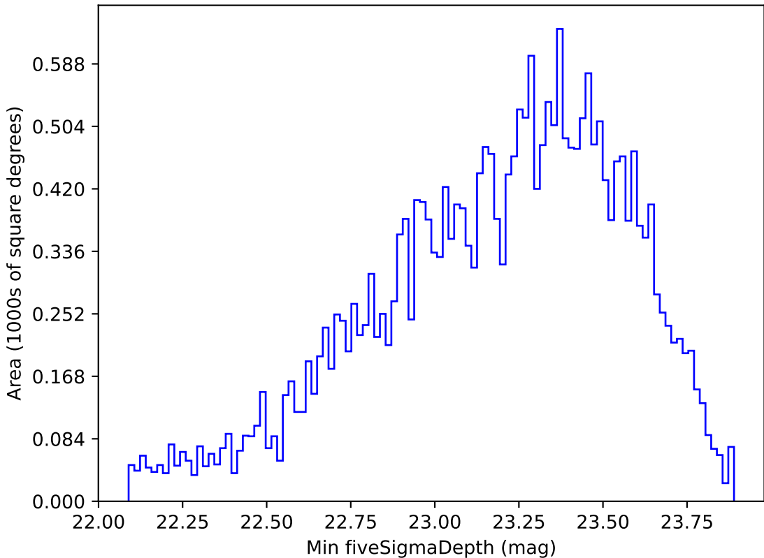
scp_reweight_v3.3_10yrs All sky g band: Min fiveSigmaDepth
