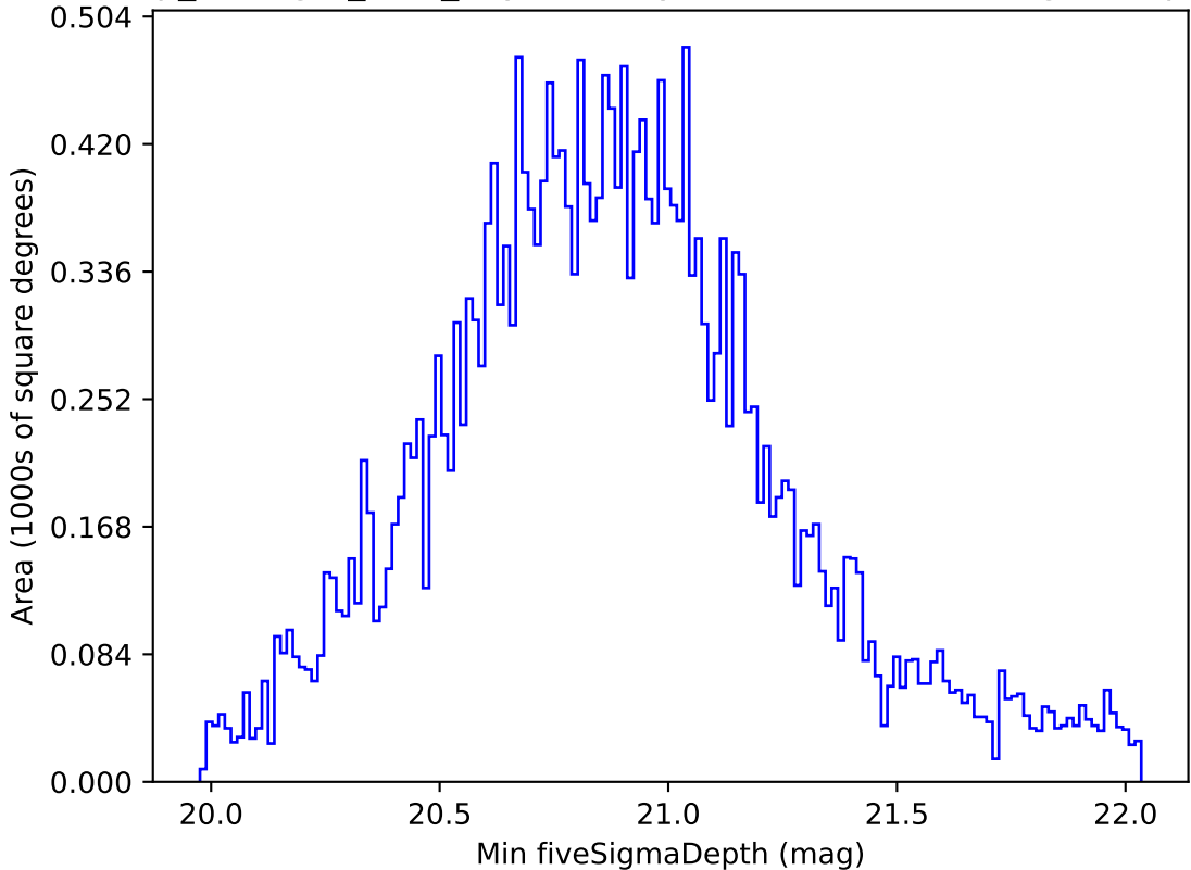
scp_reweight_v3.3_10yrs All sky all bands: Min fiveSigmaDepth
