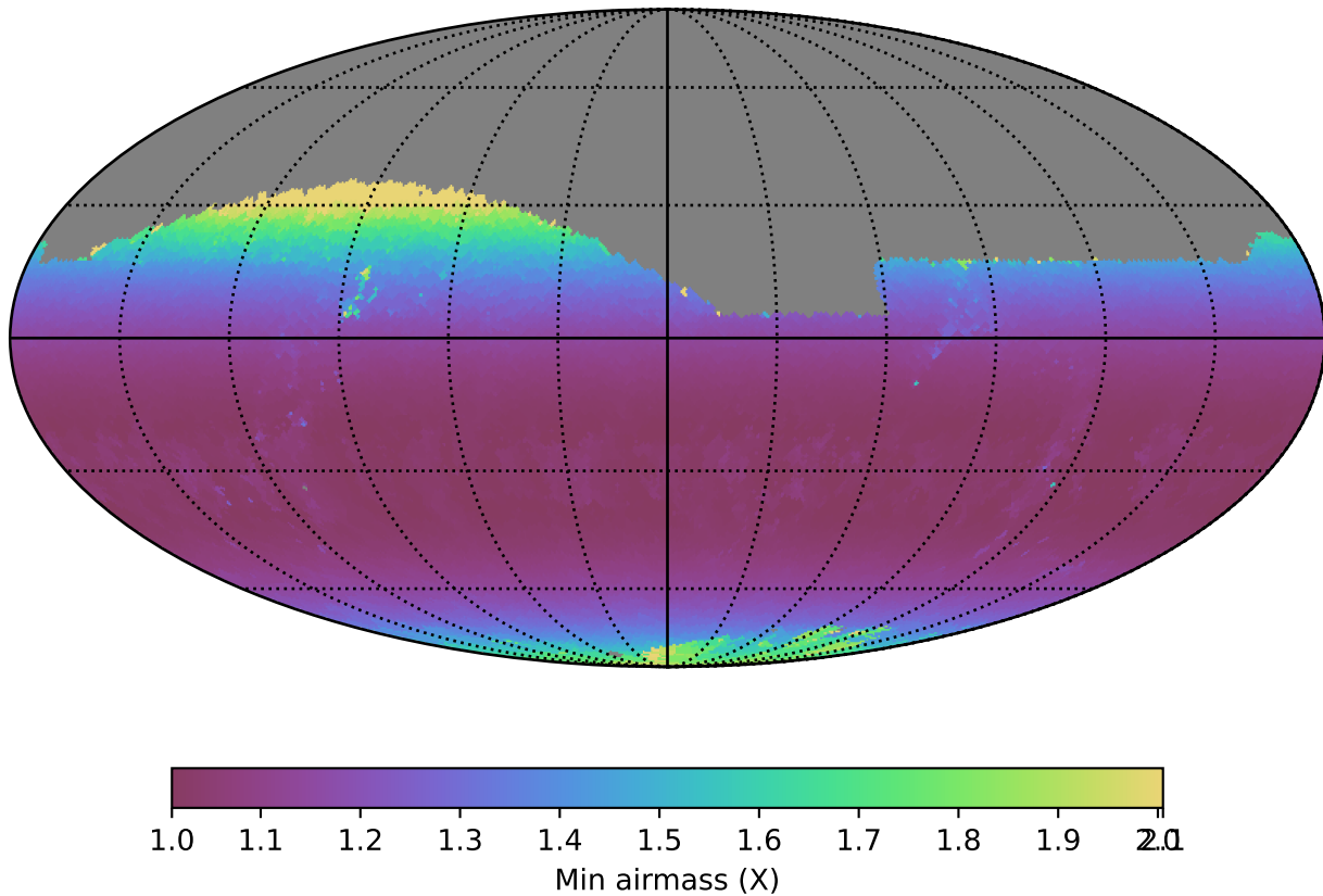
scp_reweight_v3.3_10yrs Yr 1 z band: Min airmass
