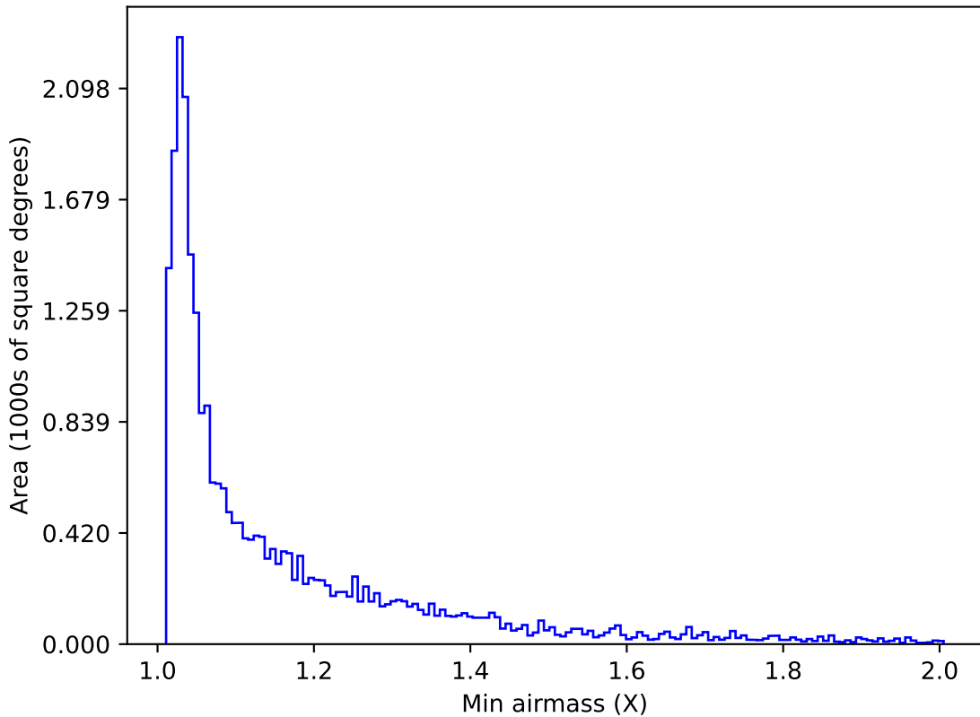
scp_reweight_v3.3_10yrs Yr 1 z band: Min airmass
