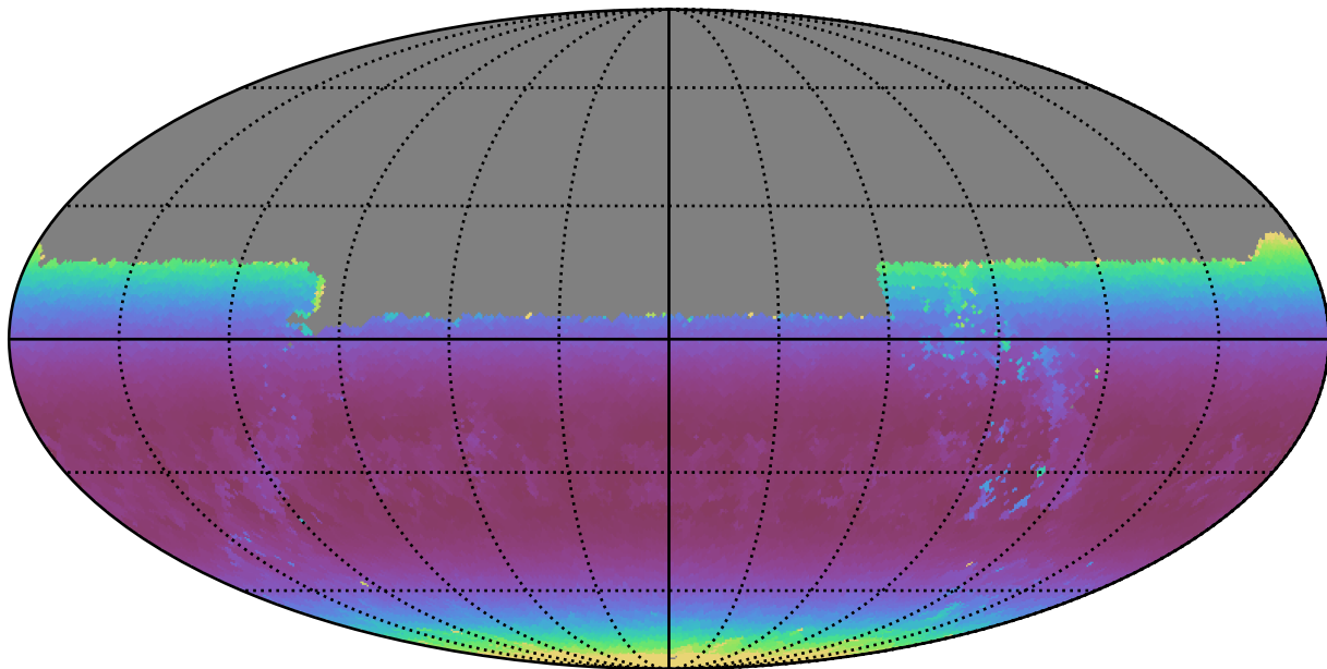
scp_reweight_v3.3_10yrs Yr 1 y band: Min airmass
