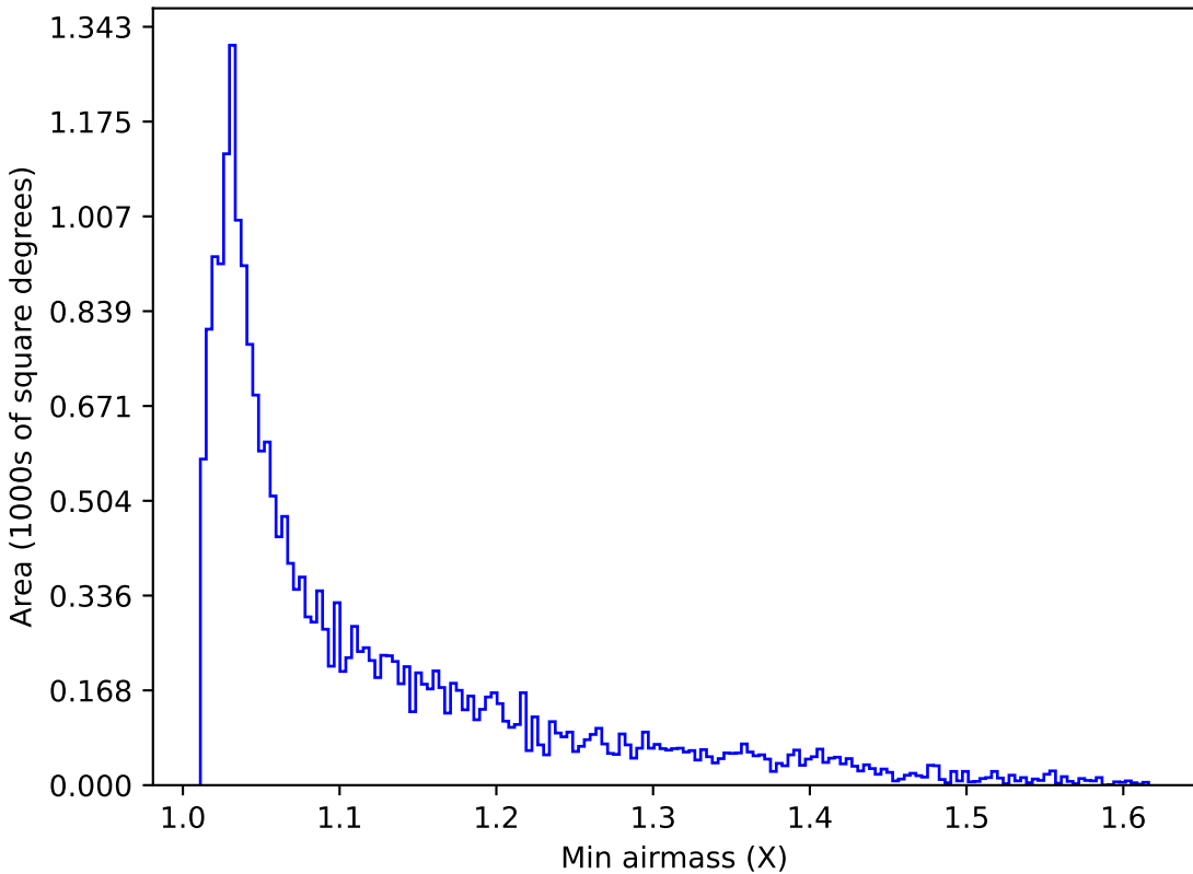
scp_reweight_v3.3_10yrs Yr 1 y band: Min airmass
