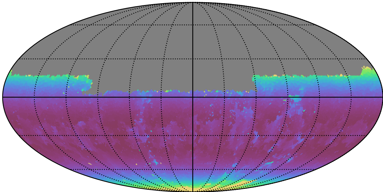
scp_reweight_v3.3_10yrs Yr 1 u band: Min airmass
