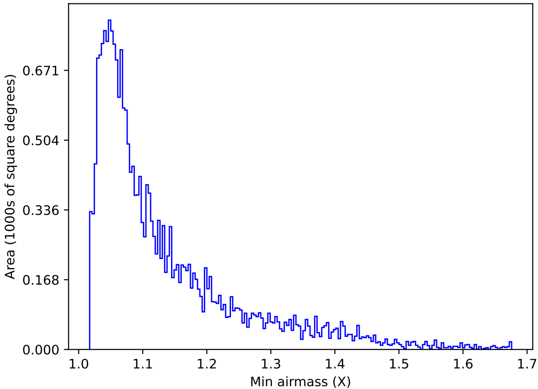
scp_reweight_v3.3_10yrs Yr 1 u band: Min airmass
