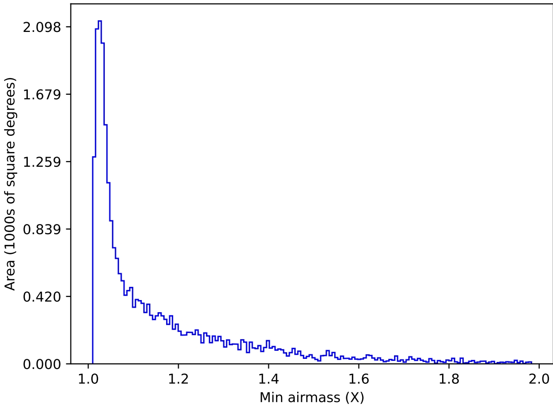
scp_reweight_v3.3_10yrs Yr 1 r band: Min airmass
