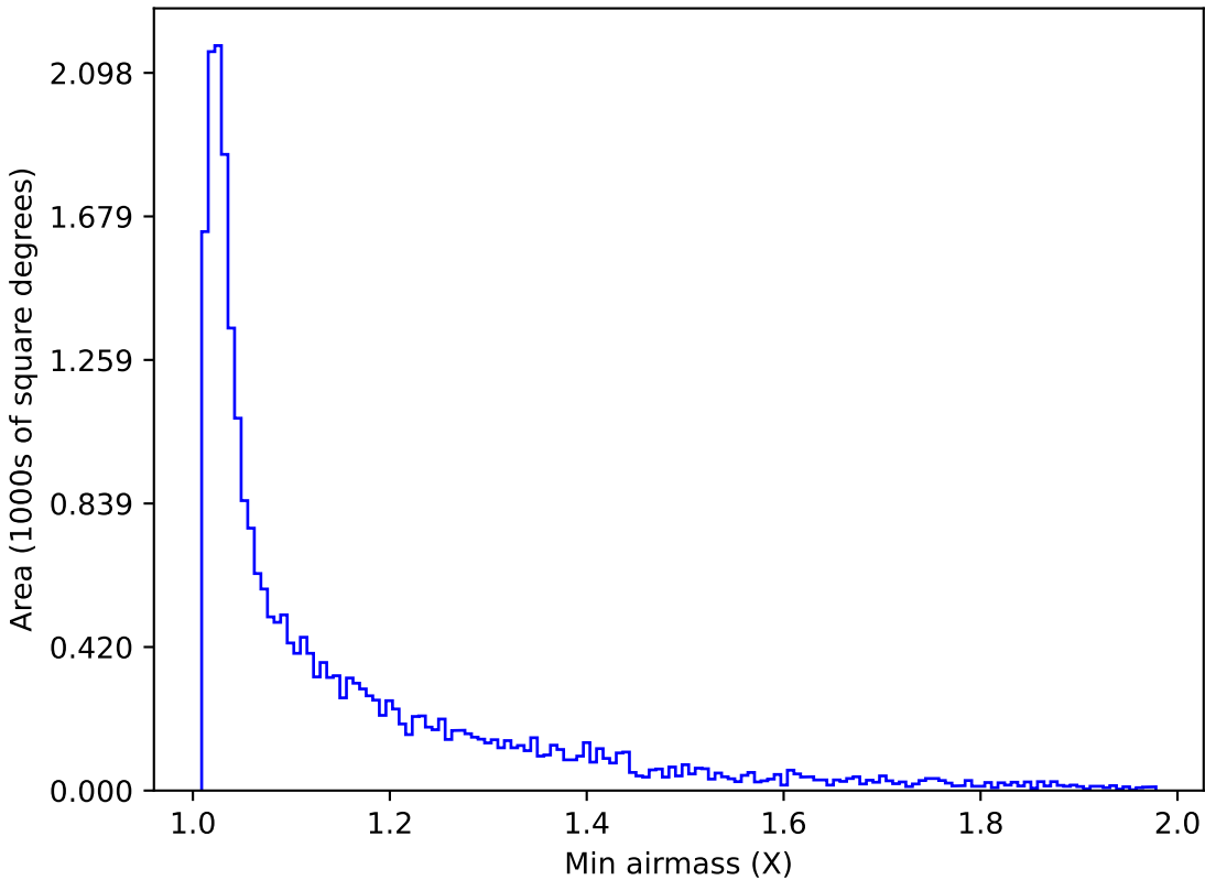
scp_reweight_v3.3_10yrs Yr 1 i band: Min airmass
