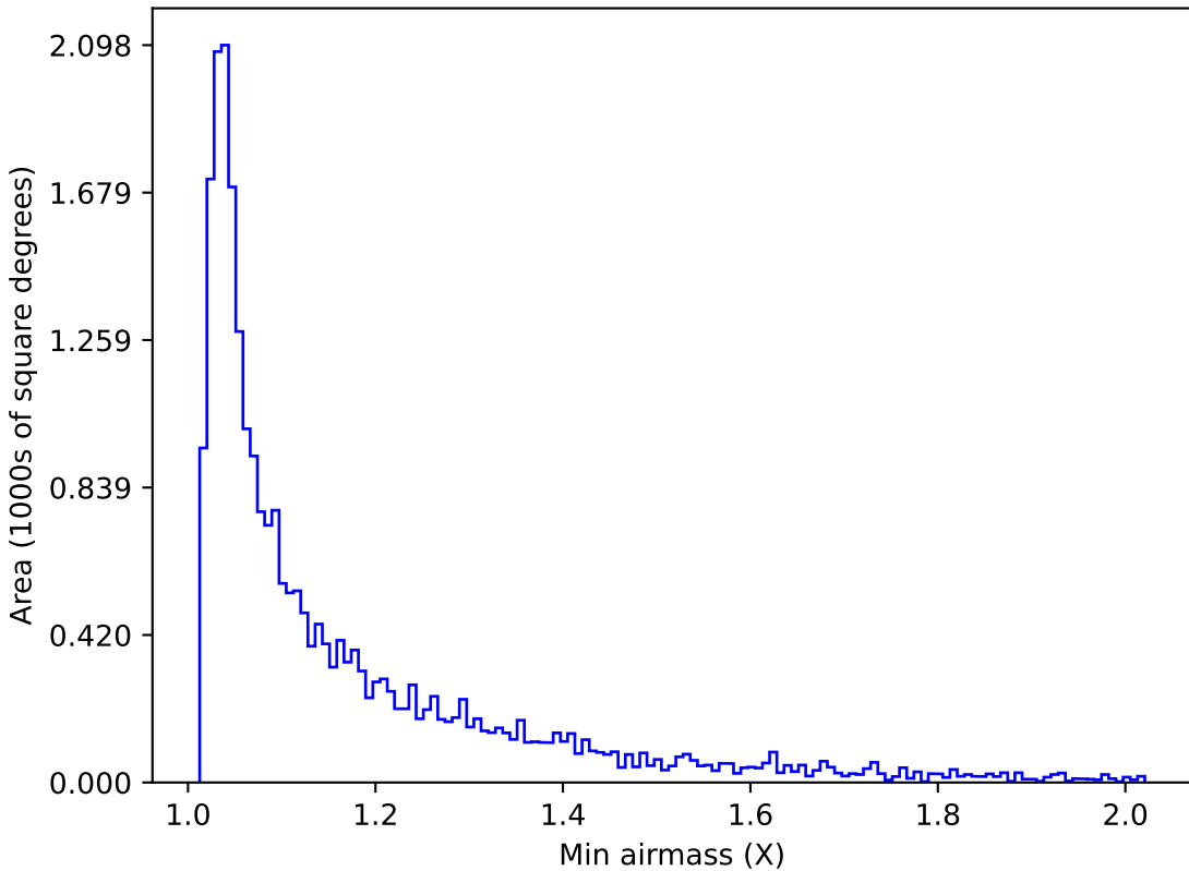
scp_reweight_v3.3_10yrs Yr 1 g band: Min airmass
