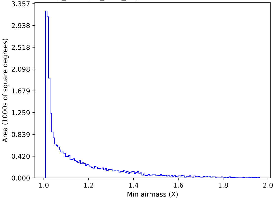
scp_reweight_v3.3_10yrs Yr 1 all bands: Min airmass
