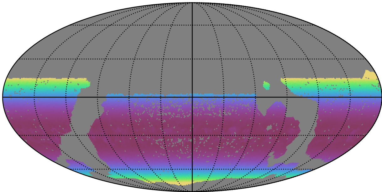
scp_reweight_v3.3_10yrs WFD z band: Min airmass
